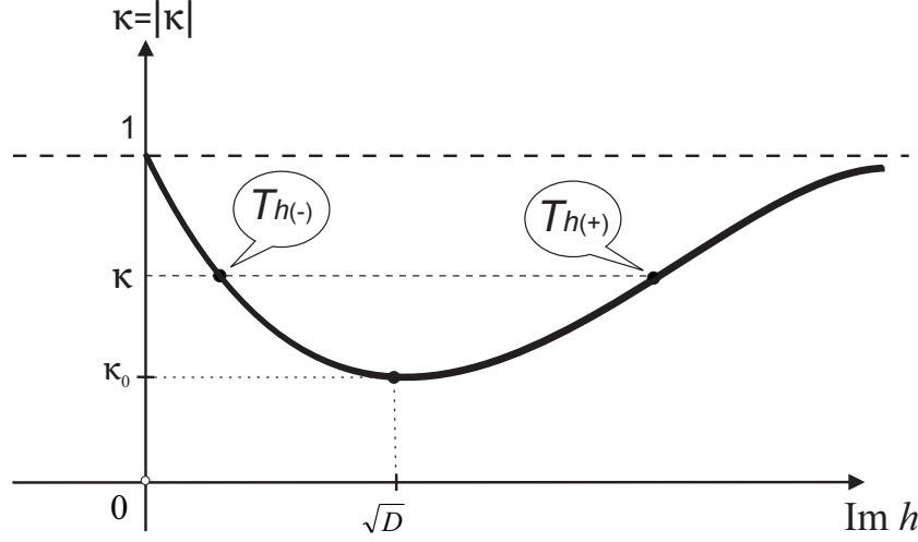
FIGURE 1. Two extremal operators T_h with the same \kappa
