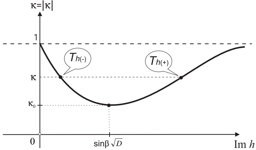
FIGURE 2. Two \beta -sectorial operators T_h with the same \kappa
